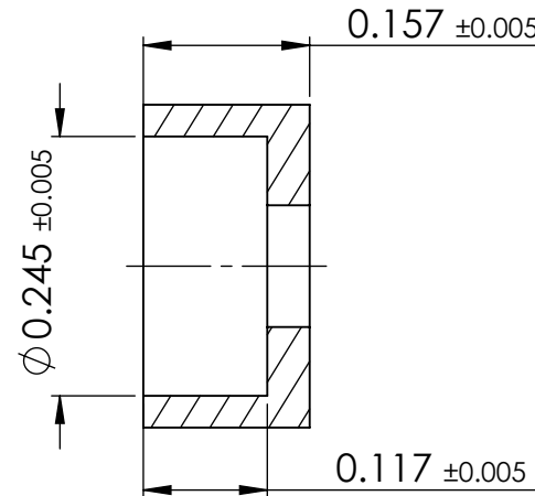
SECTION Y-Y
