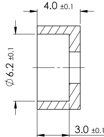
SECTION Y-Y
